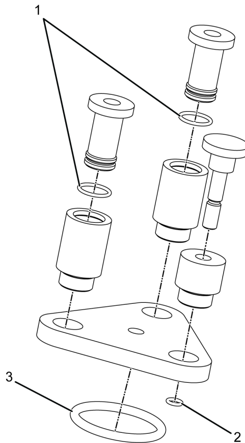
Figure 1. O-Ring Locations
