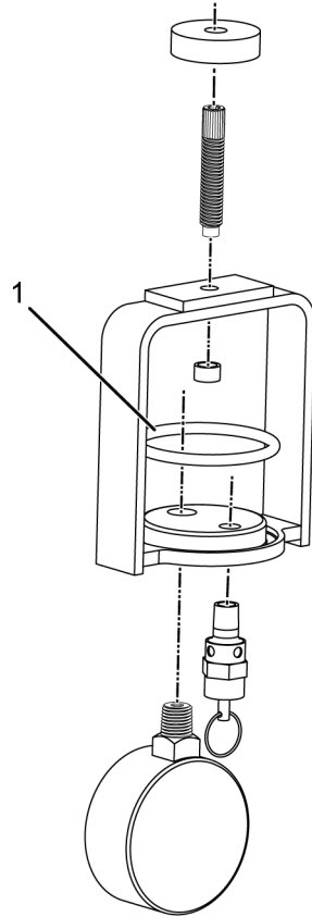
Figure 1. O-Ring Location
