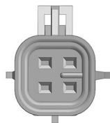
Figure 2. 12-647-02 Breakout Harness Connector View
