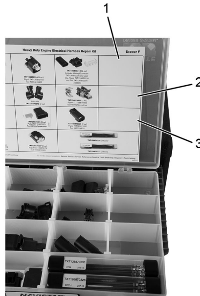
Figure 3. Connector Label Locations
