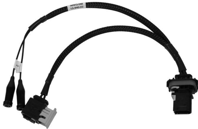
Figure 1. 13-940-02 2-Way Breakout Harness
